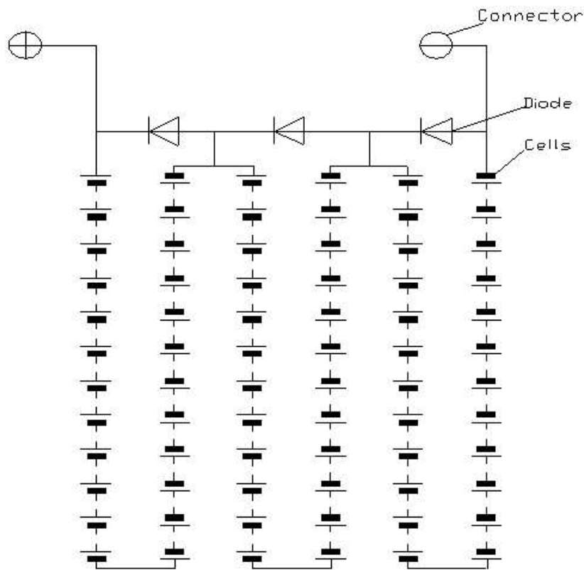
Circuit diagram
